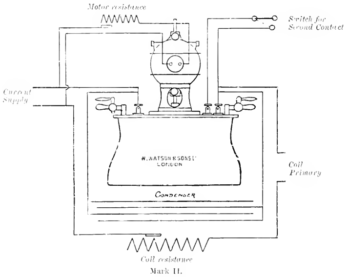
FIG. 13.—Plan of connections for Dreadnought interrupter.
